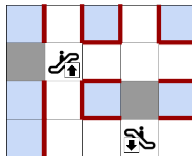
One optimal way of installing windows for the first sample case. The blue cells are the shops. The red edges are the windows.
